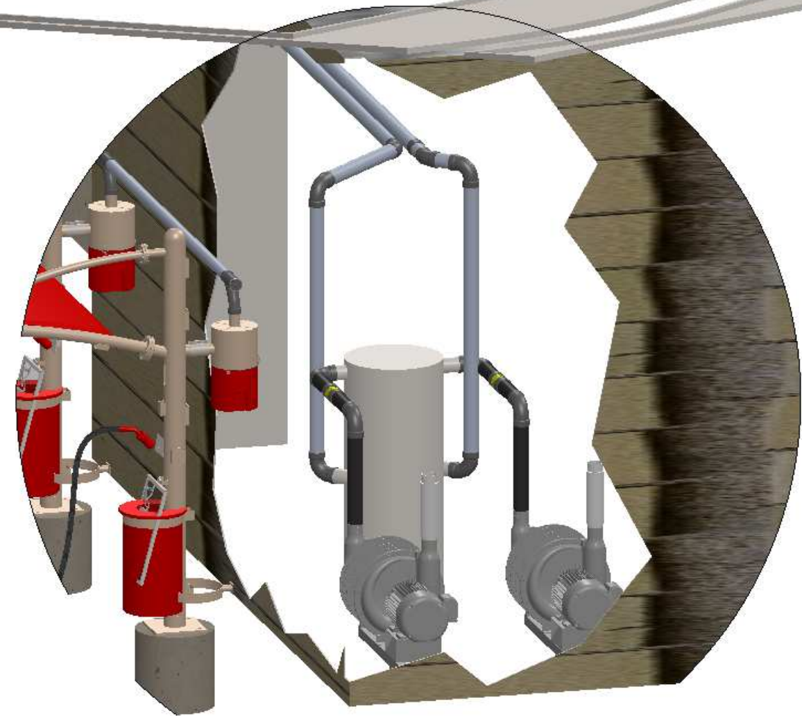
VACUUM PRODUCER DETAIL
