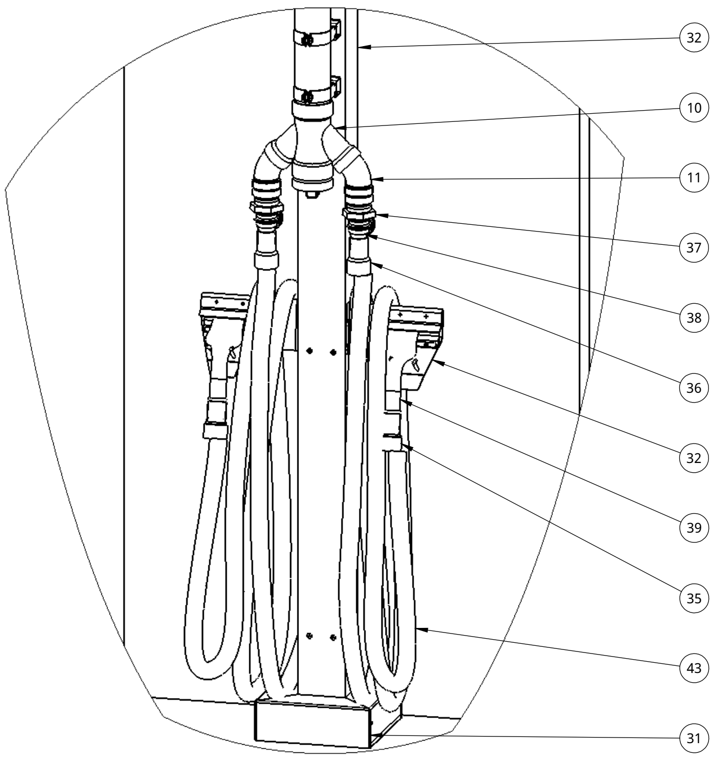
DETAIL B
