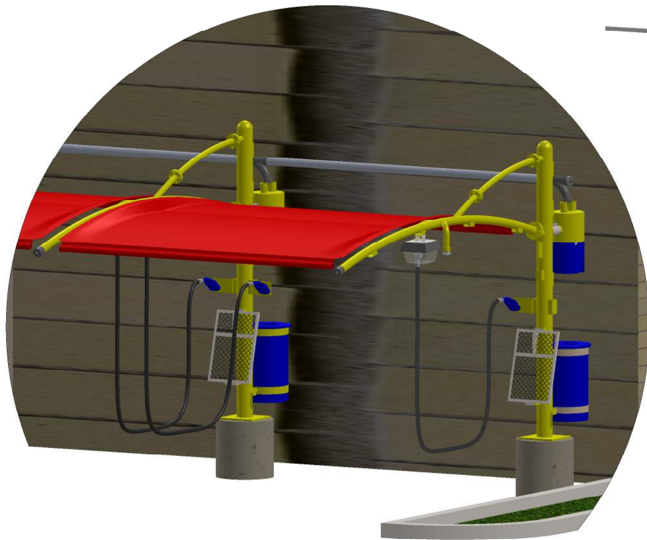
VACUUM ARCH DETAIL
