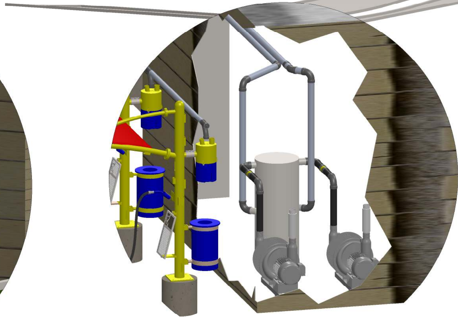
VACUUM PRODUCER DETAIL
